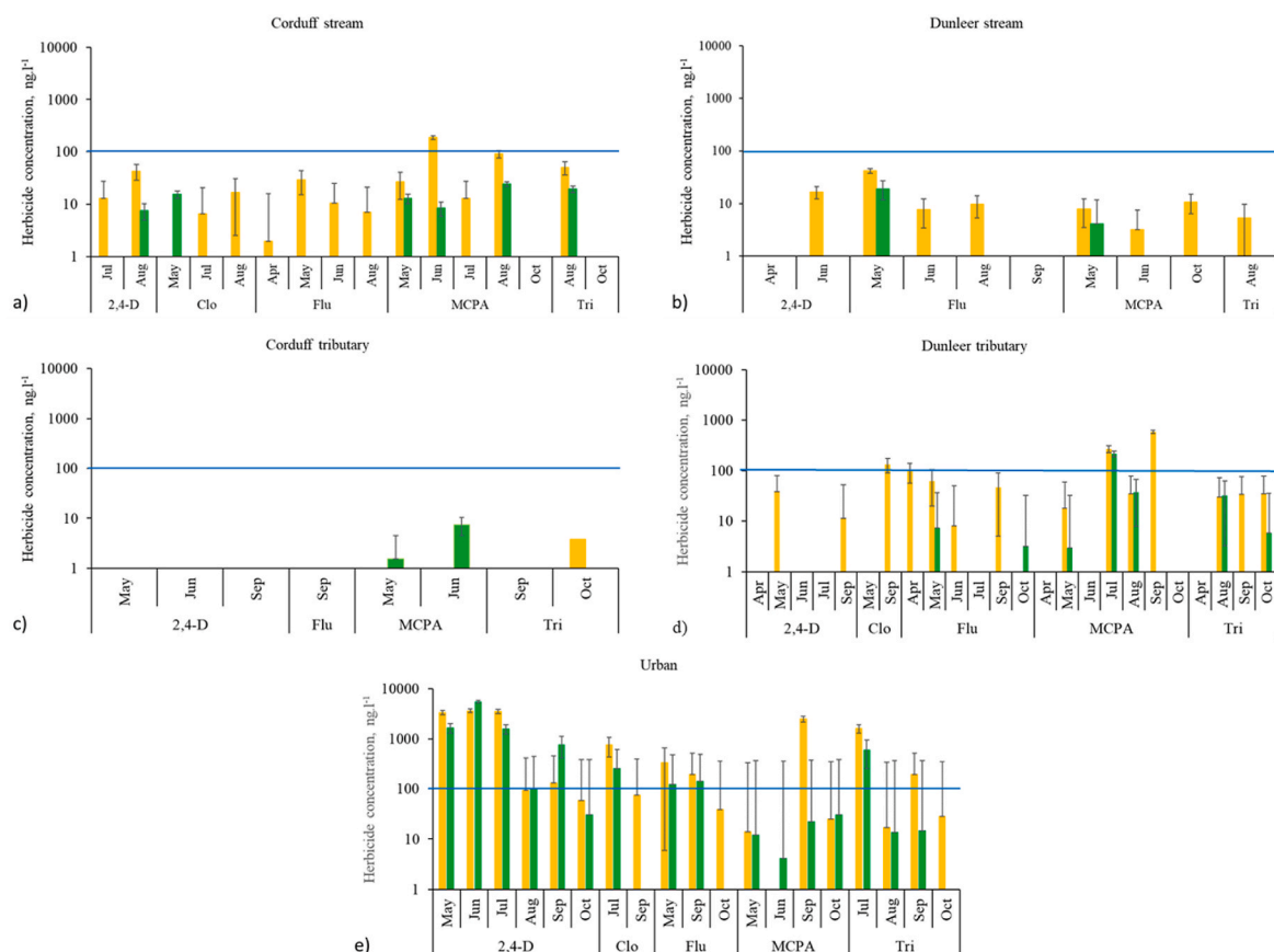
Fig. 5. Herbicide detections for the filter pipe interventions across all sampling areas. Clo = clocyralid, Flu = fluroxypyr and Tri = triclopyr. Yellow columns indicate herbicide concentrations before the filter pipe interventions, and green columns indicate herbicide concentrations after the filter pipe interventions. Average values of the two Chemcatchers® have been displayed for each monthly detection. Error bars show standard error where n = 2 . The blue line is the maximum allowable concentration for individual herbicides (100 ng l -1 ). (For interpretation of the references to colour in this figure legend, the reader is referred to the Web version of this article.)
