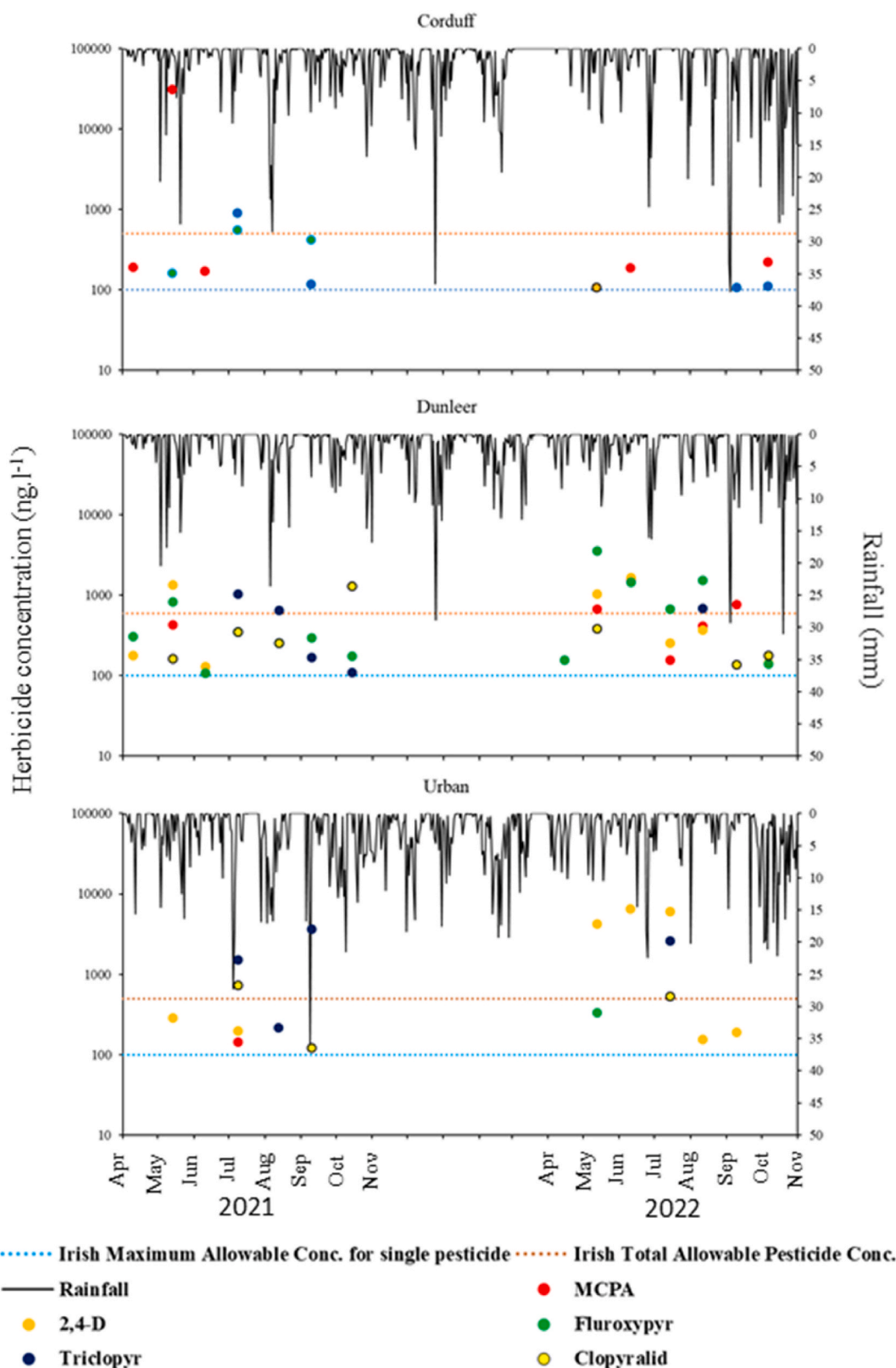
Fig. 3. Exceedances of herbicides at outlet points in Corduff, Dunleer and Urban sampling areas for Year 1 (2021) and Year 2 (2022) of the study.
