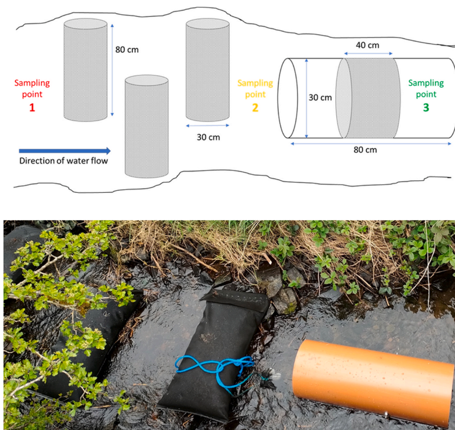
Fig. 2. Schematic of different configurations of the intervention positioned in the stream. The blue arrow indicates direction of water flow. Filter bags are upstream from the filter pipe. Sampling points, colour-coded (see Section 2.4), are also indicated on the scheme. Photo shows actual configurations in one of the streams, with first bag of three in the top left hand corner of photo. (For interpretation of the references to colour in this figure legend, the reader is referred to the Web version of this article.)
