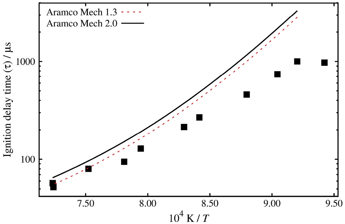
C_2H_4 in Air, \Phi = 0.5, p_{av} = 1.0 atm
