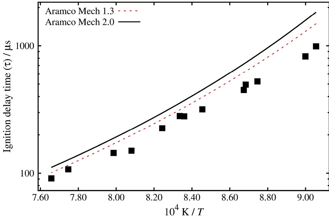
C_2H_4 in Air, \Phi = 0.3, p_{av} = 1.0 atm
