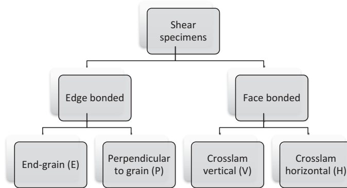
FIGURE 1 Schema of specimen configurations for shear tests.
