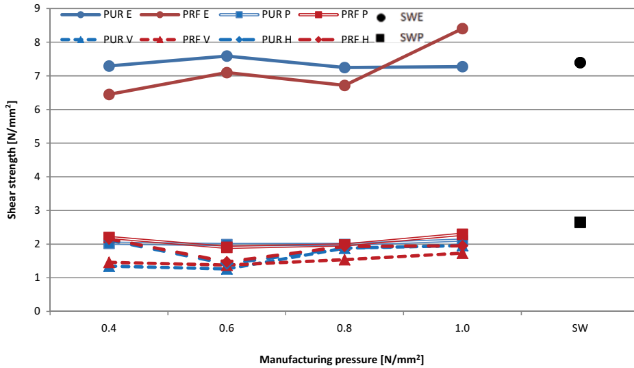
FIGURE 5 Five-percentile shear strength values for different test configurations.
