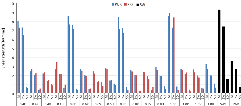
FIGURE 3 Shear strength values*.
