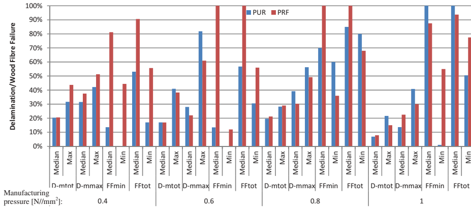
FIGURE 4 Delamination tests results † .
