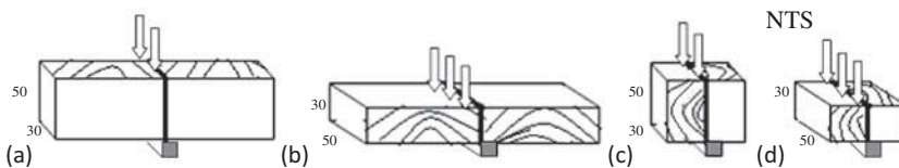
FIGURE 2 Shear test specimens for: (a) end-grain, (b) perpendicular to grain loading, and crosslam bonded elements vertically (c) and horizontally (d) loaded (dimensions in millimetres).
