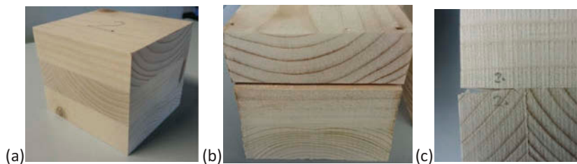
FIGURE 8 Specimen for delamination test (a) before and after vacuum-pressure cycle (b, c).
