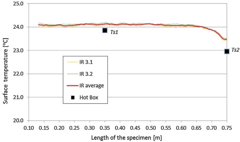
Fig. 12. Surface temperatures of Specimen 3.
