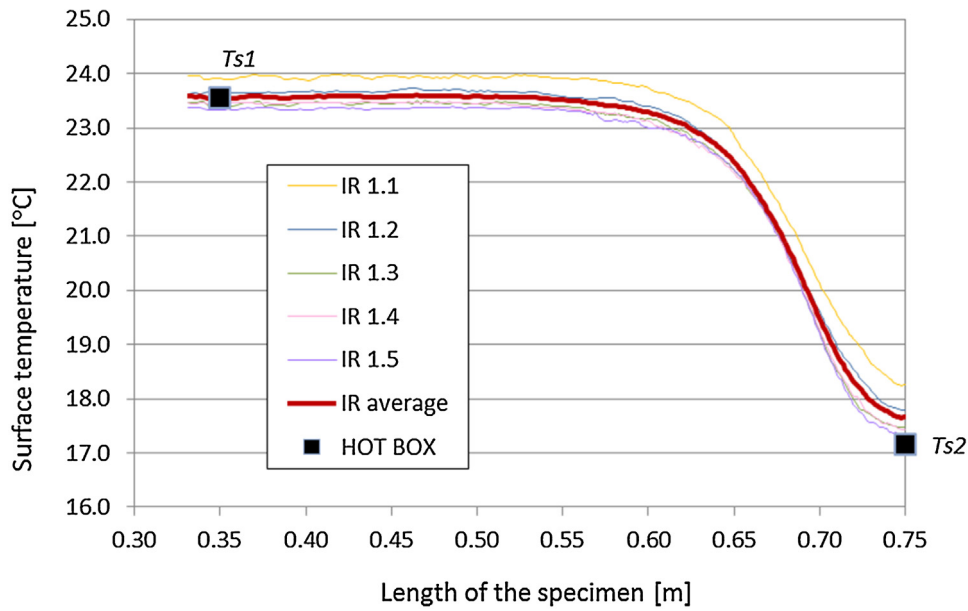
Fig. 10. Surface temperature of Specimen 1.
