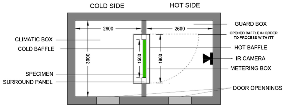
Fig. 4. Experimental set up.
