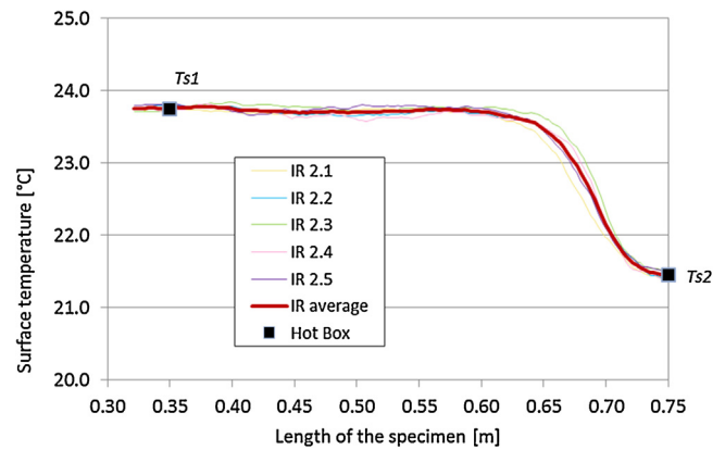
Fig. 11. Surface temperature of Specimen 2.
