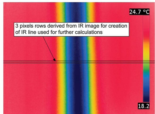
Fig. 2. Sample IR image of component with linear thermal bridge.
