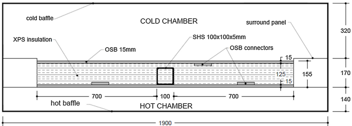
Fig. 6. Cross-section of Specimen 2 inserted in hot box.
