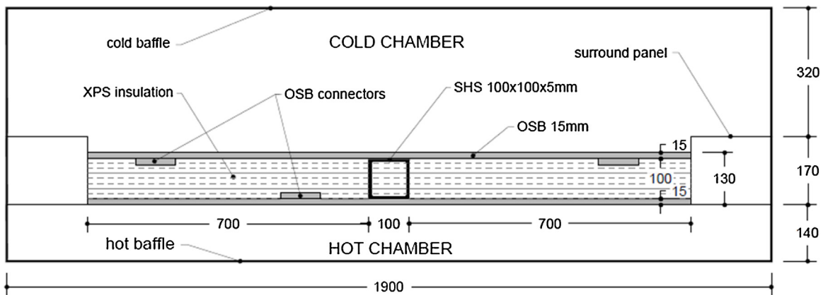
Fig. 5. Cross-section of Specimen 1 inserted in hot box.
